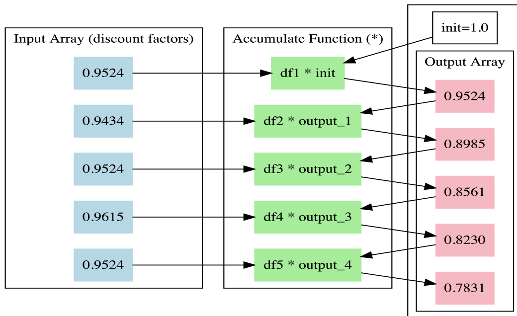
Figure 6.2.: A diagram showing that accumulate creates a new collection where each element is the cumulative result of applying the given operation to all previous elements.
