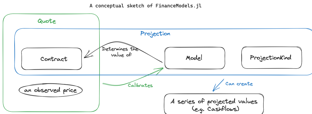
Figure 8.1.: A conceptual sketch of FinanceModels.jl components.
