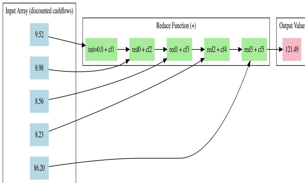
Figure 6.3.: A diagram showing how reduce applies the given operation to pairs of elements, ultimately reducing the collection to a single value.
