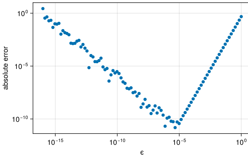
Figure 16.1.: A log-log plot showing the absolute error of the finite differences. Further to the left, roundoff error dominates while further to the right, truncation error dominates.
