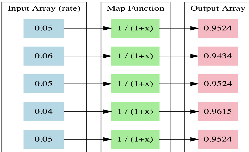
Figure 6.1.: A diagram showing that map creates a new collection mirroring the old one, after applying the given function to each element in the original collection.
