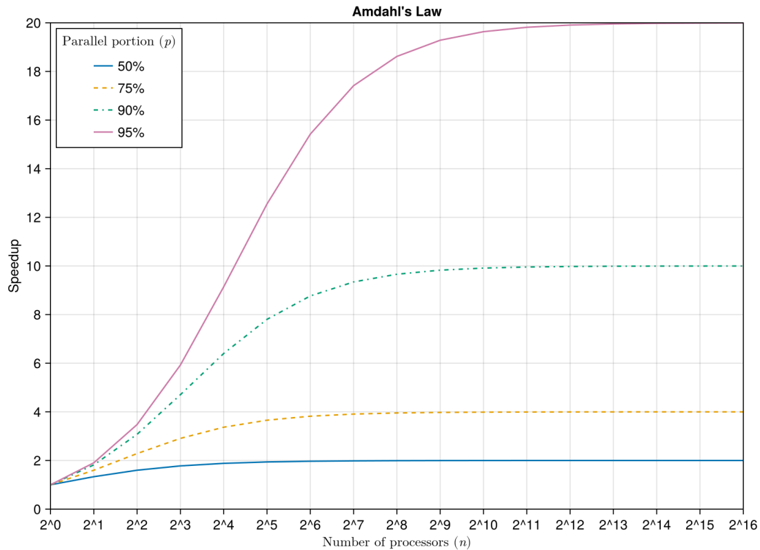
Figure 11.1.: Theoretical upper bound for speedup of a workload given the parallelizable portion p and number of processors n .
